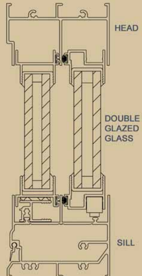
DG 300 Cross Section
